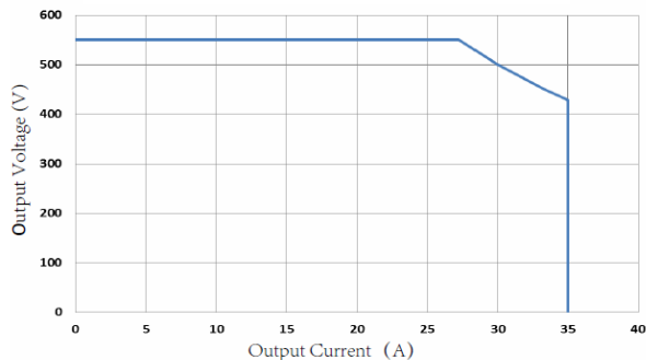
C750-20H-Output Voltage VS. Output Current
